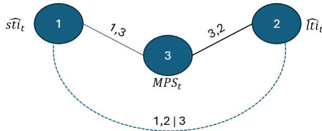
Figure 2: Hierarchical copula structure in a chain.
