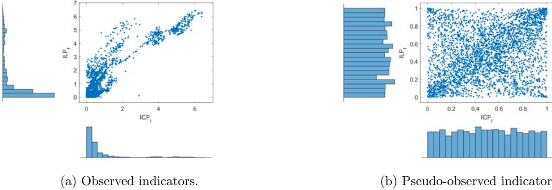
Figure 5: Comparison of raw vs transformed indicators
