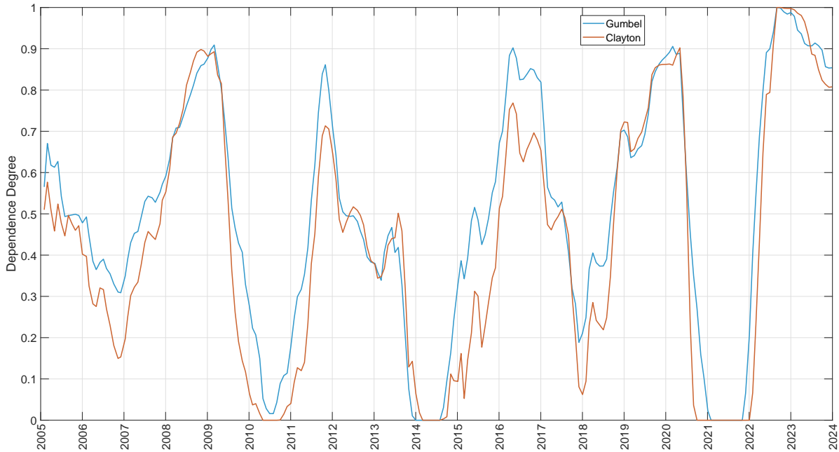
(b) Positive dependency
