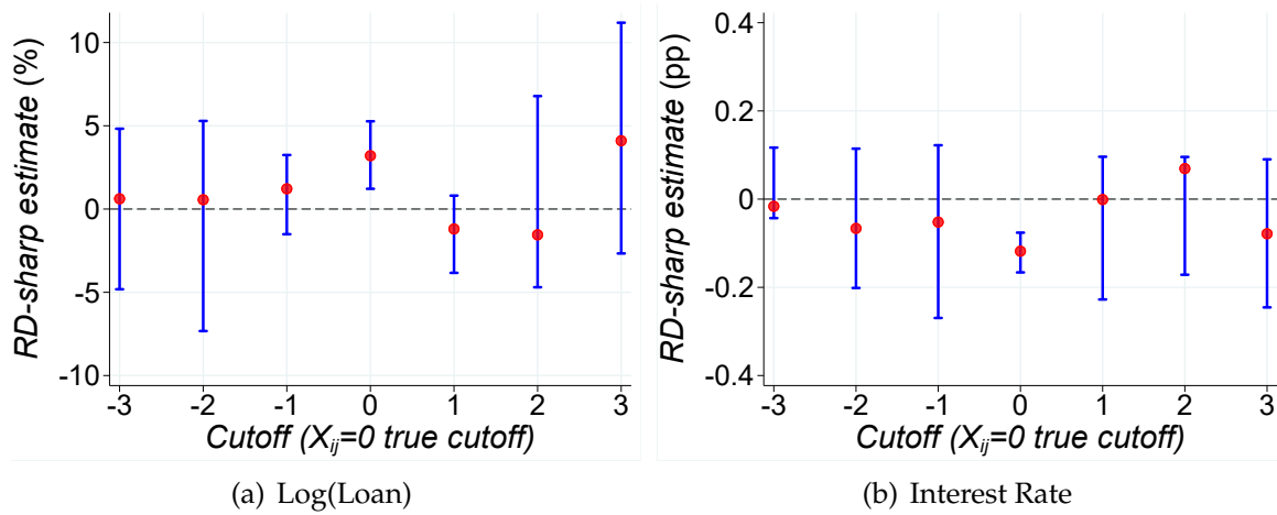
Figure 4: Placebo cutoffs
