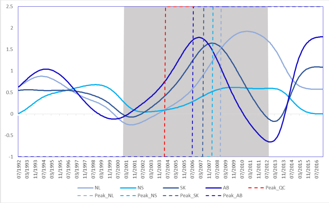
Figure 4: Time-varying contagion coefficients
