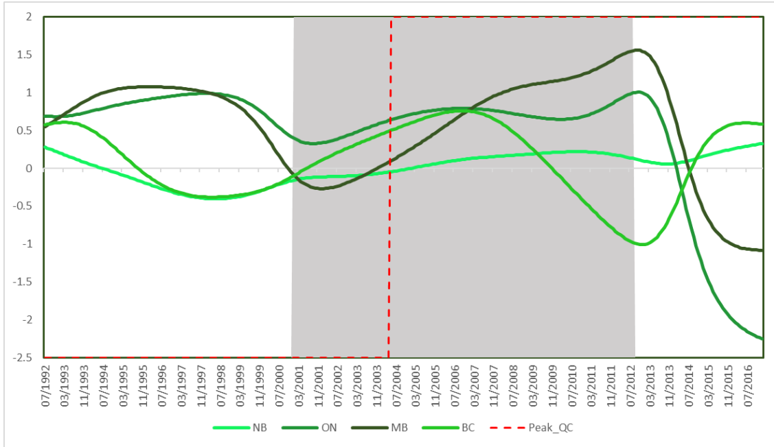
Figure 5: Time-varying contagion coefficients
