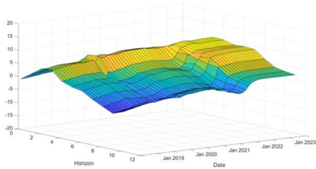
Figure 6: Response of CDS for a panel of emerging market countries to a one standard deviation shock in the GPR index using recursive estimations.
