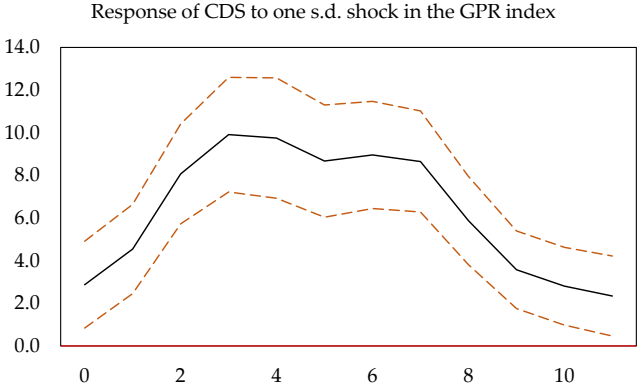
Figure 3: Response of CDS for a panel of emerging market countries to a one-standard deviation shock in the GPR index. The dotted line represents the 68% confidence bands.
